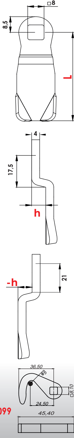
Pano Kilit Dilleri Panel Locks Cams
