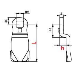
Paslanmaz Diller Stainless Steel Cams
